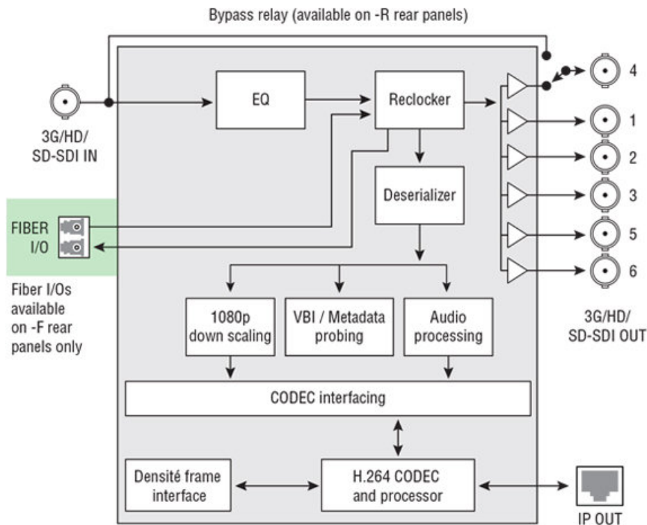
SME-1901 Functional Block Diagram
